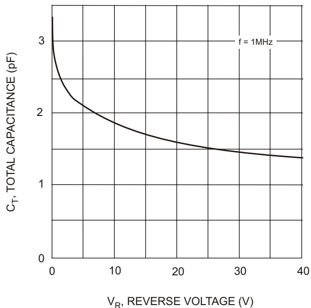
Fig. 3 Typical Capacitance
