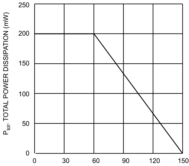
T A - AMBIENT TEMPERATURE (°C) Fig. 1 Total Power Dissipation vs. Ambient Temperature
