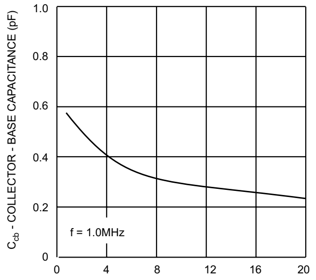
V CB - COLLECTOR - BASE VOLTAGE (V) Fig. 2 Collector - Base Capacitance vs. Collector - Base Voltage
