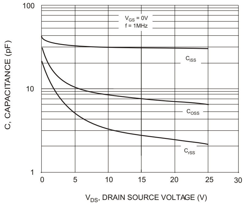
Fig. 10 Capacitance vs. Drain Source Voltage
