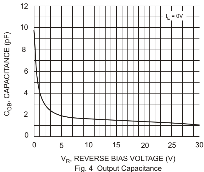
Fig. 4 Output Capacitance
