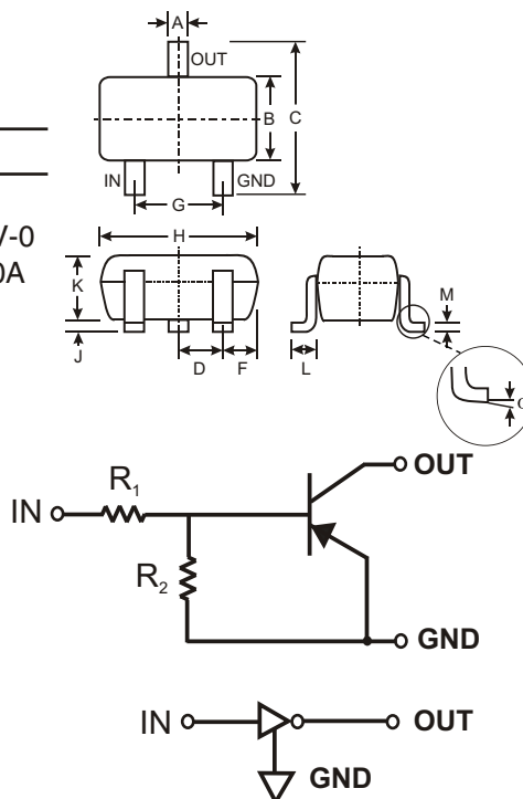
SCHEMATIC DIAGRAM
