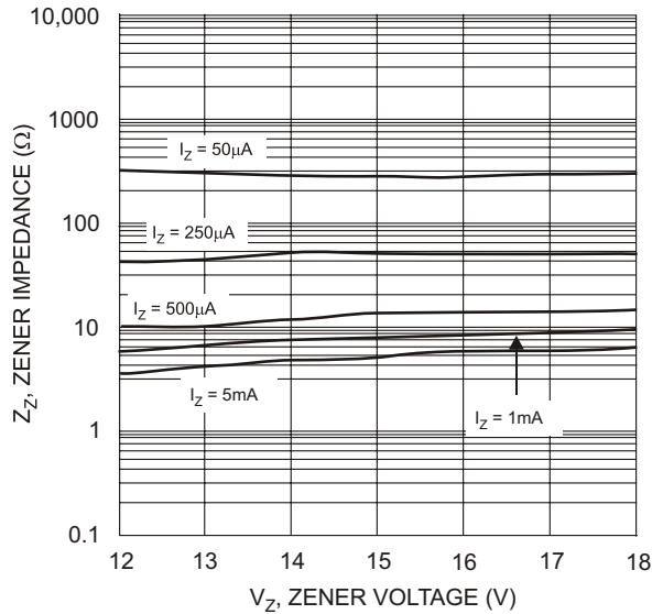
Fig. 12 Typical Zener Impedance Characteristics, DDZ9699 - DDZ9705
