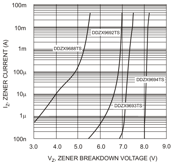
Fig. 4 Typical Reverse Characteristics, DDZX9688TS - DDZX9694TS
