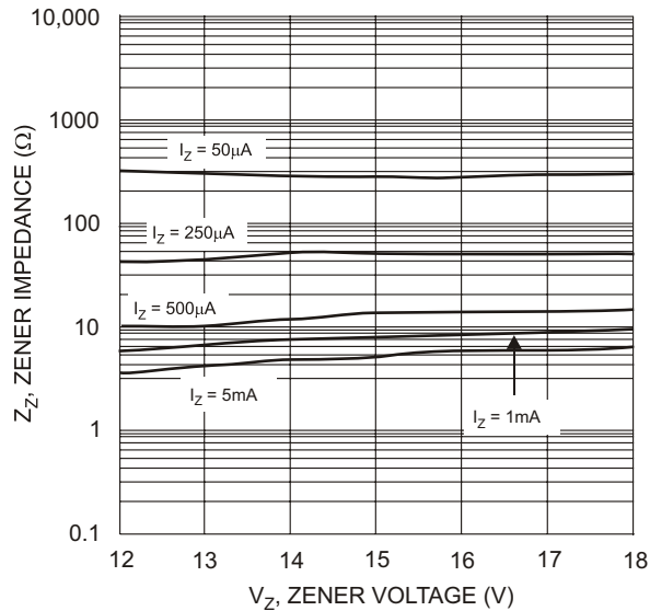
Fig. 12 Typical Zener Impedance Characteristics, DDZX9699TS - DDZX9705TS
