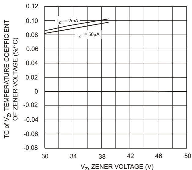
Fig. 19 Typical Temperature Coefficient of Zener Voltage, DDZ9713S - DDZ9716S
