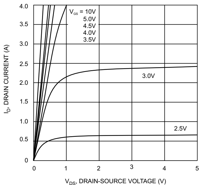
Fig. 1 On-Region Characteristics
