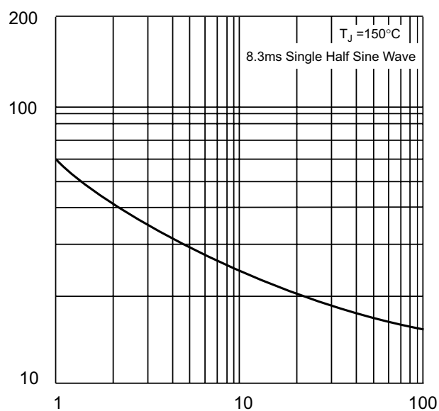
I_F , PEAK FWD SURGE CURRENT (A) Fig. 4 Peak Forward Surge Current
