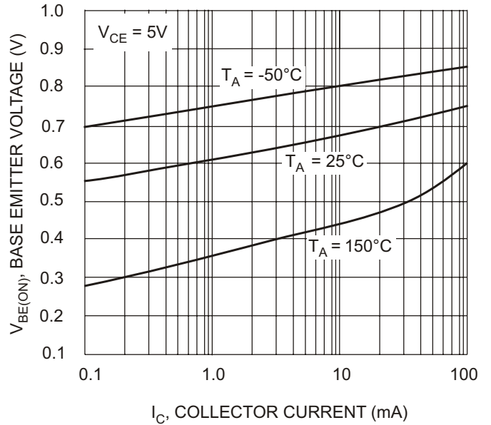
Fig. 4, Base Emitter Voltage vs. Collector Current
