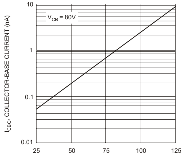
Fig. 2 Typical Collector-Cutoff Current vs. Ambient Temperature
