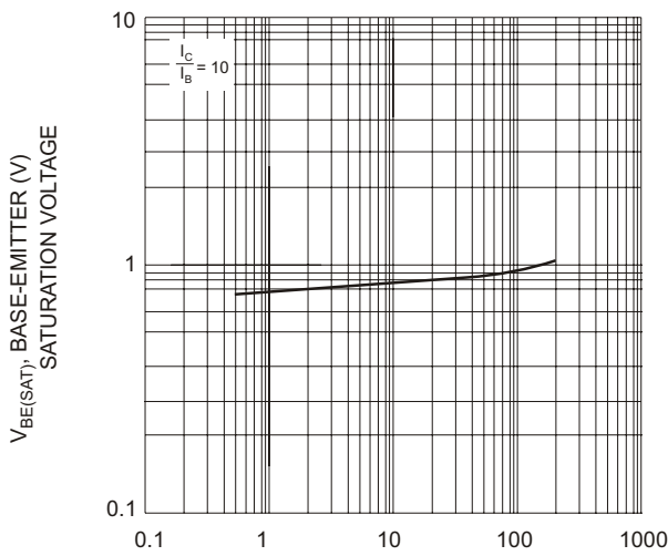
V_{BE(SAT)} , BASE-EMITTER SATURATION VOLTAGE I_C , COLLECTOR CURRENT (mA) Fig. 5, Typical Base-Emitter Saturation Voltage vs. Collector Current (NPN-3904)
