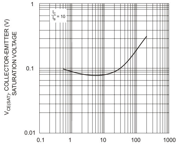
V_{CE(SAT)} , COLLECTOR-EMITTER SATURATION VOLTAGE I_C , COLLECTOR CURRENT (mA) Fig. 4, Typical Collector-Emitter Saturation Voltage vs. Collector Current (NPN-3904)
