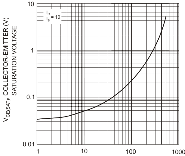
I_C, \text{ COLLECTOR CURRENT (mA)} Fig. 4, Typical Collector-Emitter Saturation Voltage vs. Collector Current
