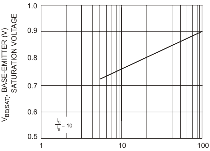
I_C, \text{ COLLECTOR CURRENT (mA)} Fig. 5, Typical Base-Emitter Saturation Voltage vs. Collector Current
