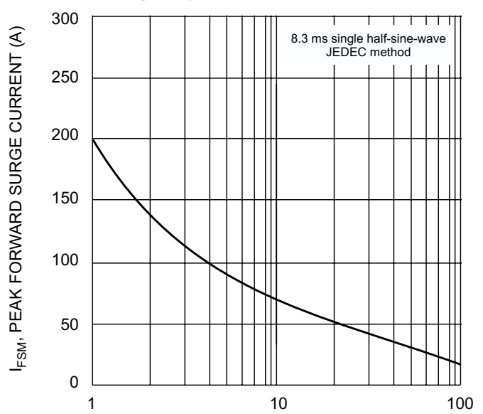
NUMBER OF CYCLES AT 60Hz Fig. 4 Maximum Non-Repetitive Surge Current
