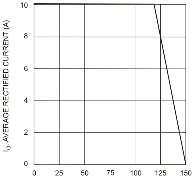
T_C , CASE TEMPERATURE (°C) Fig. 1 Forward Derating Curve
