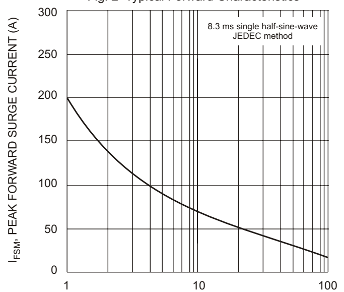
8.3 ms single half-sine-wave JEDEC method Fig. 4 Maximum Non-Repetitive Surge Current
