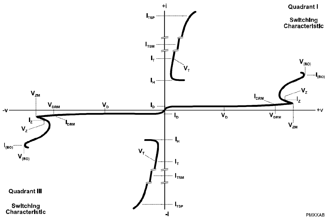
Figure 1. VOLTAGE-CURRENT CHARACTERISTIC FOR ANY PAIR TERMINALS
