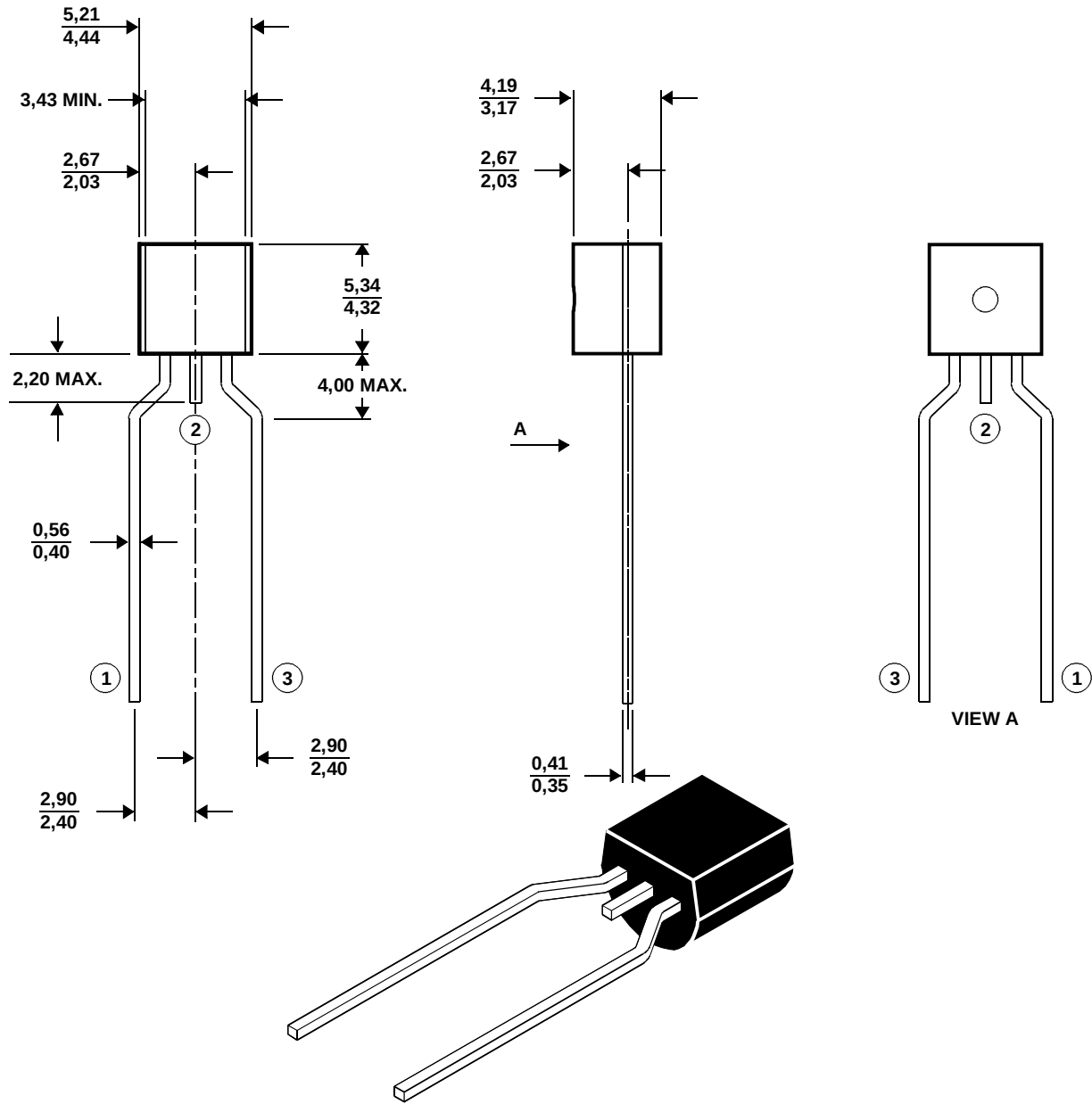
LMF002 (DO-92) - Formed Leads Version of LM002
