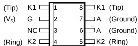
'61060D PACKAGE (TOP VIEW)
