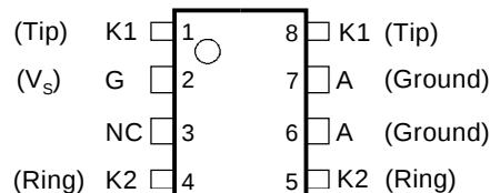
'61060P PACKAGE (TOP VIEW)
