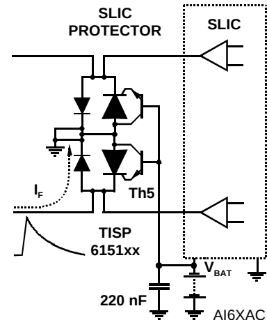
Figure 5. POSITIVE OVERVOLTAGE CONDITION
