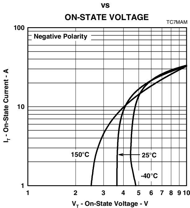
TISP7125F3 THRU TISP7180F3 ON-STATE CURRENT
