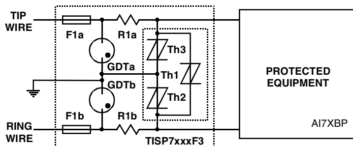
Figure 36. PROTECTION MODULE
