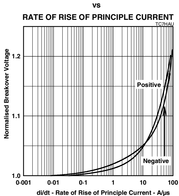
TISP7240F3 THRU TISP7380F3 NORMALISED BREAKOVER VOLTAGE
