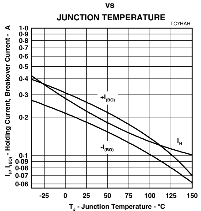
HOLDING CURRENT & BREAKOVER CURRENT
