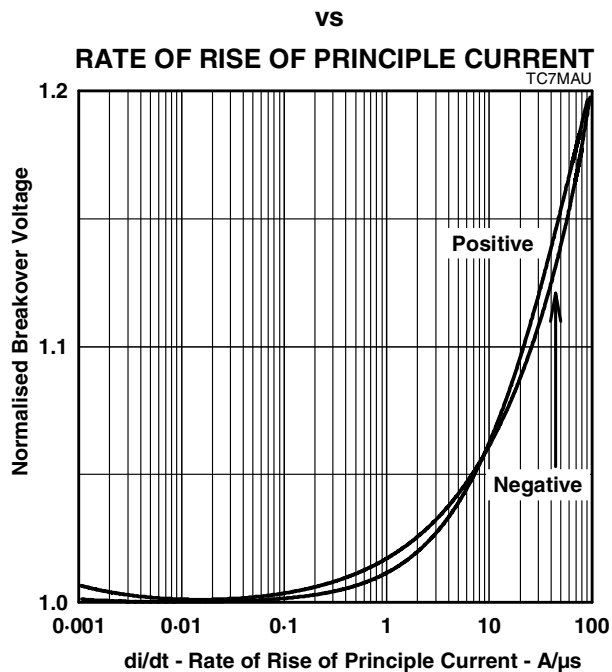
TISP7125F3 THRU TISP7180F3 NORMALISED BREAKOVER VOLTAGE
