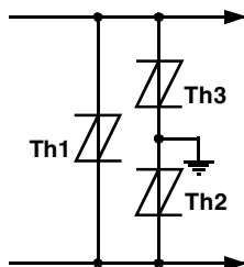
Figure 32. MULTI-POINT PROTECTION
