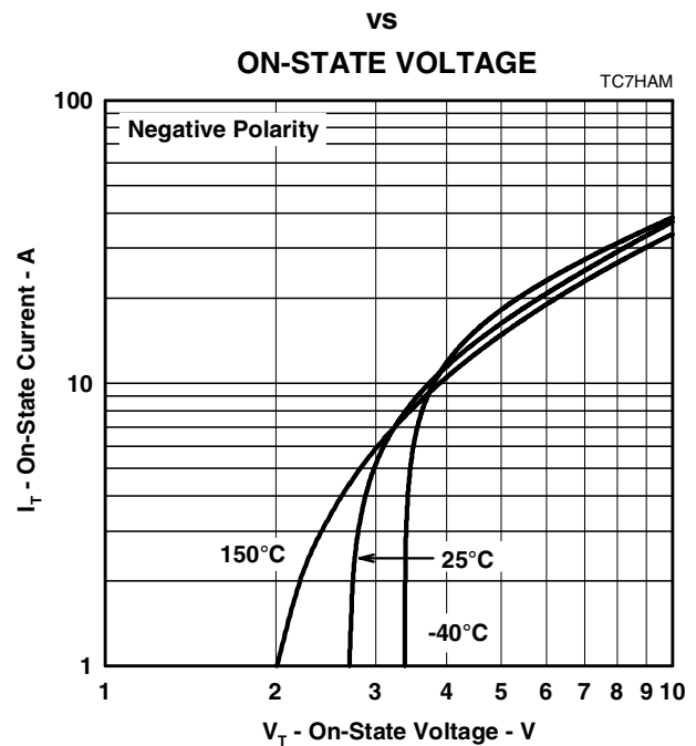
TISP7240F3 THRU TISP7380F3 ON-STATE CURRENT
