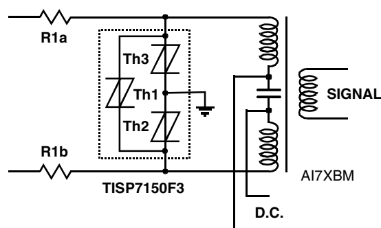
Figure 37. ISDN PROTECTION
