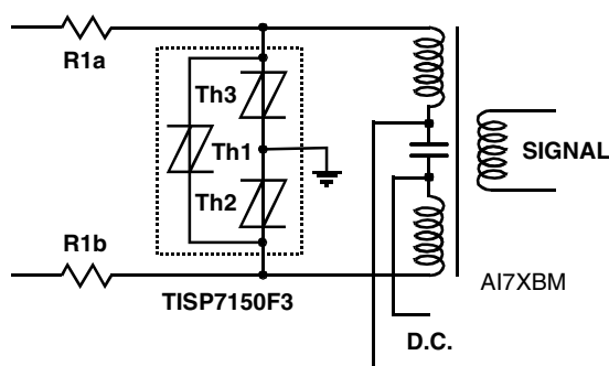
Figure 37. ISDN PROTECTION
