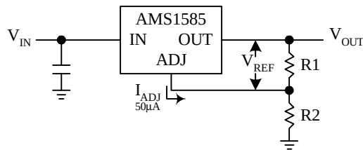
Figure 1. Basic Adjustable Regulator
