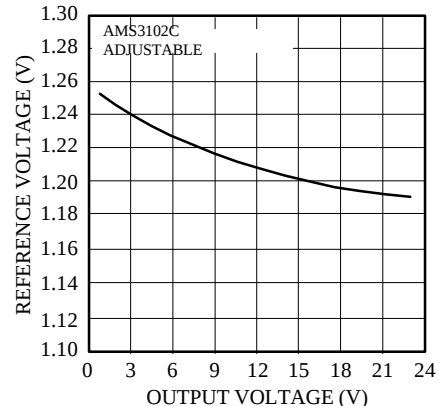
Reference Voltage
