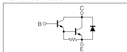
Internal Connection
