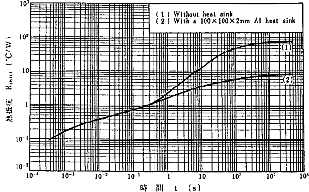
R_{th(t)} - t
