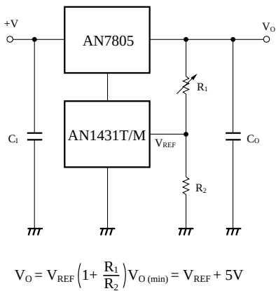
5.Adjustable Output Regulator Combined with 3-pin Regulator
