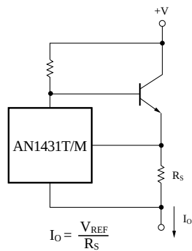
3.Constant Current Source
