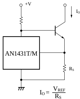
2.Constant Current Power Supply
