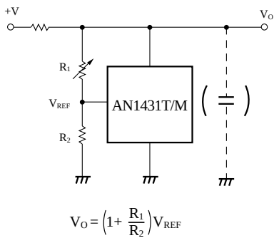
1.Shunt Regulator
