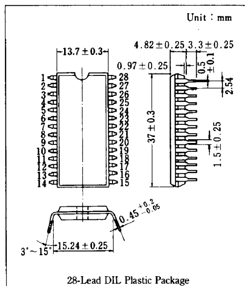
28-Lead DIL Plastic Package
