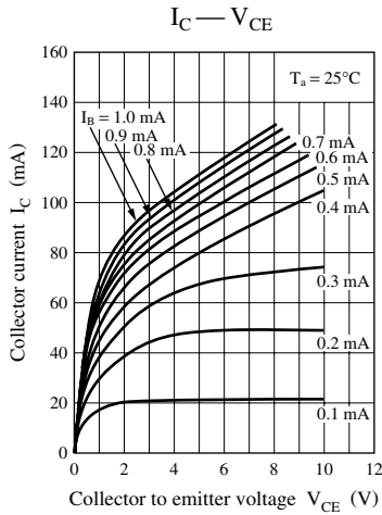
Characteristics chart of UNR9212J
