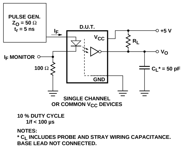
Figure 9. Switching Test Circuit.*
