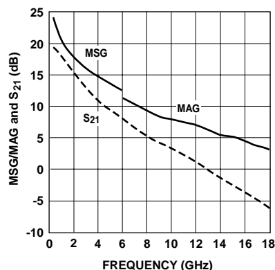
Figure 20. MSG/MAG and |S_{21}|^2 vs. Frequency at 2 V, 20 mA.
