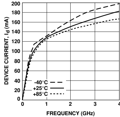
Figure 10. Supply Current vs. Voltage and Temperature. P_{in} = -27\text{ dBm} .
