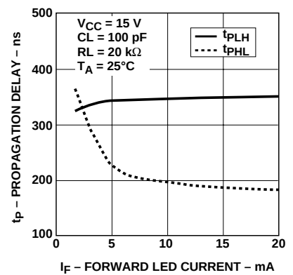
Figure 17. Propagation Delay vs. Input Current.
