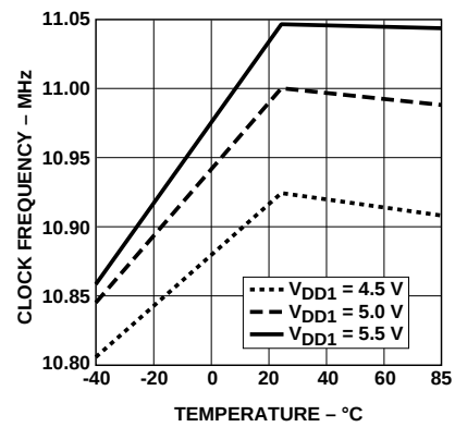
Figure 17. Clock Frequency vs. Temperature.
