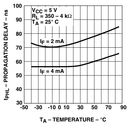
Figure 9. t_{\text{PHL}} – Propagation Delay vs. Temperature.
