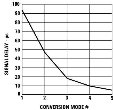
Figure 13. Signal Delay vs. Conversion Mode.
