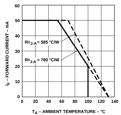
Figure 4a. Maximum DC Current vs. Ambient Temperature for AS T-1 3/4 Lamps. Derating Based on T_{jMAX} = 130^{\circ}\text{C} .
