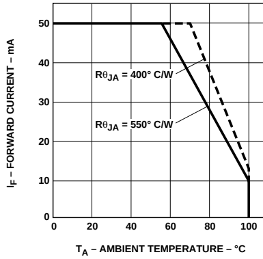
Figure 12. Maximum Forward Current vs. Ambient Temperature. Derating Based on T_J Max = 110^{\circ}\text{C} .
