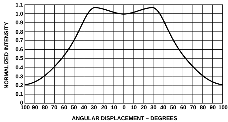
Figure 7. Relative luminous intensity vs. angular displacement for 125° device.
