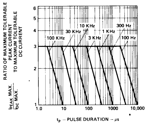
Figure 15. Maximum Tolerable Peak Current vs. Pulse Duration. ( I_{\text{DC MAX}} as per MAX Ratings).
