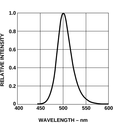
Figure 1. Relative intensity vs. wavelength.
