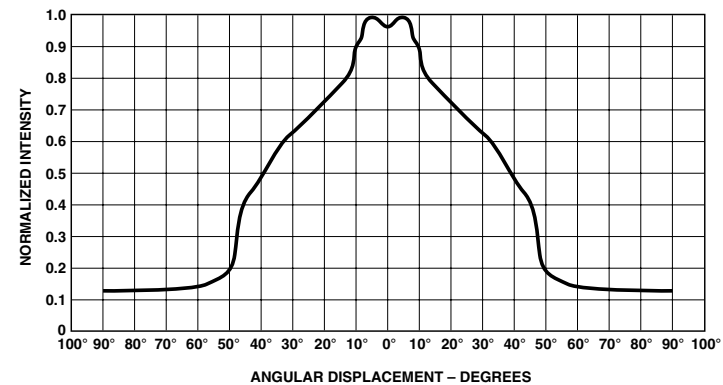
Figure 10. HLMP-P106/-P156.
