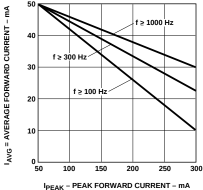
Figure 7. Maximum Average Current vs. Peak Forward Current.
