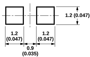
Figure 10. Recommended soldering pattern for HSMx-C170.
