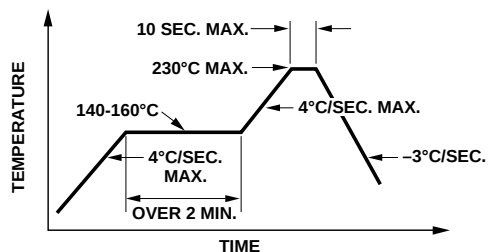
Figure 7. Recommended reflow soldering profile.
