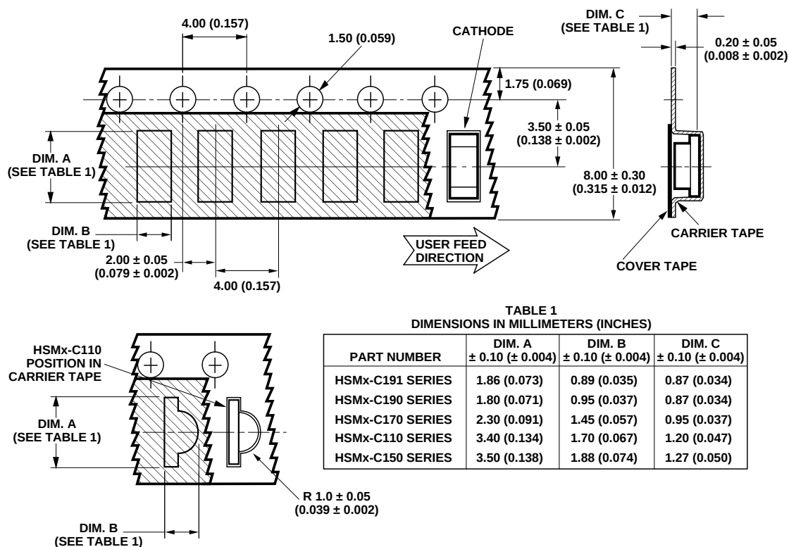
Figure 15. Tape dimensions.
