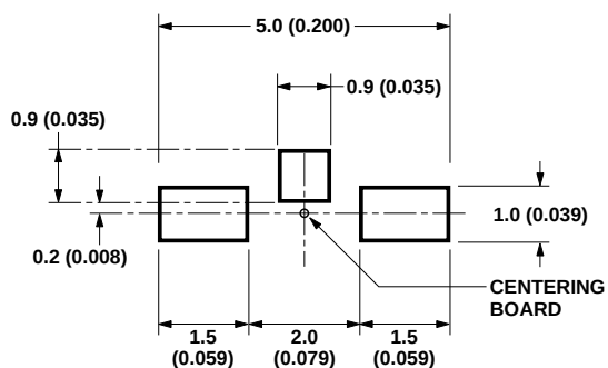
Figure 9. Recommended soldering pattern for HSMx-C110.
