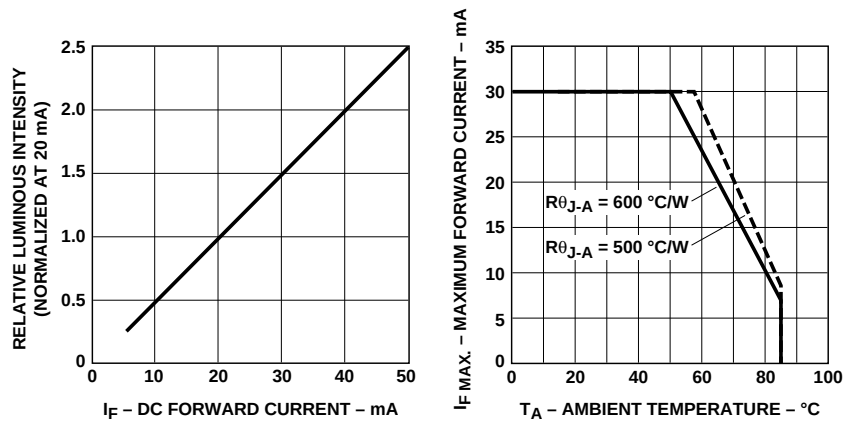
Figure 3. Relative Luminous Intensity vs. Forward Current.
