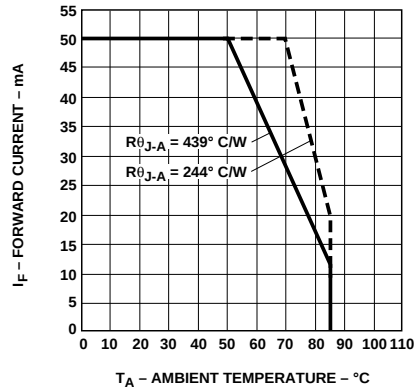
Figure 4. Maximum Forward Current vs. Ambient Temperature. Derating Based on T_J Max = 95°C.
