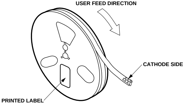
Figure 8. Reeling Orientation.
