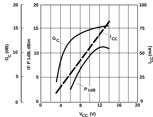
Figure 3. Typical Conversion Gain, IF P_{1dB} , and I_{CC} Current vs. V_{CC} Bias Voltage, T_A = 25^\circ\text{C} , RF: -20 dBm at 2 GHz, LO: 0 dBm at 1.75 GHz.
