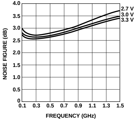
Figure 2. Noise Figure vs. Frequency and Voltage.
