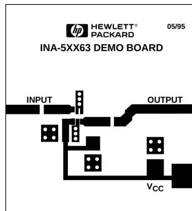
Figure 12. RF Layout.
