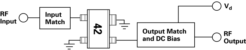
Figure 1. Block Diagram of Test Fixture. See Figure 7 in the Applications section for an equivalent schematic of 1.9 GHz circuit; Figure 11 in the Applications section for 900 MHz circuit.
