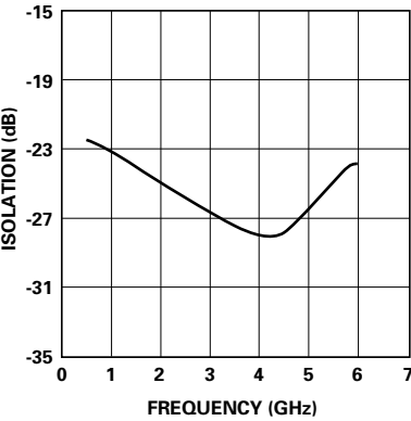
Figure 22. Isolation vs. Frequency.
