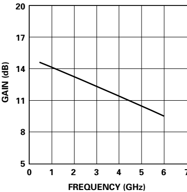
Figure 20. Gain vs. Frequency.
