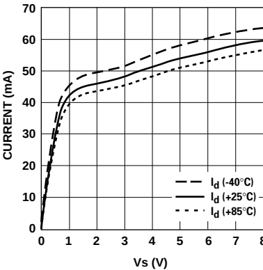
Figure 24. Current vs. Vd.
