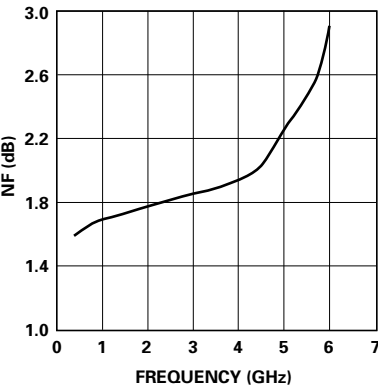
Figure 19. Noise Figure vs. Frequency (in 50Ω).
