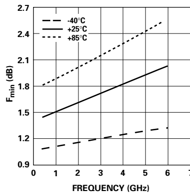
Figure 4. Minimum Noise Figure vs. Frequency and Temperature [1] .
