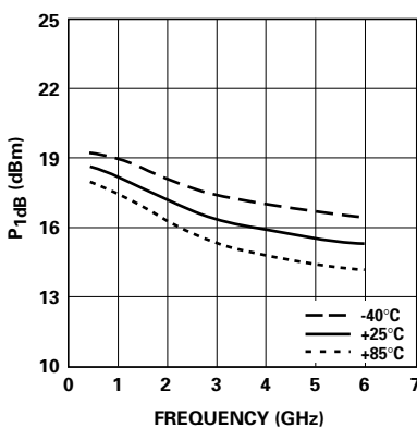
Figure 15. Output Power at 1 dB Compression vs. Frequency and Temperature.
