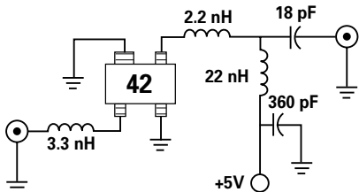
Figure 7. Schematic of 1.9 GHz Circuit.
