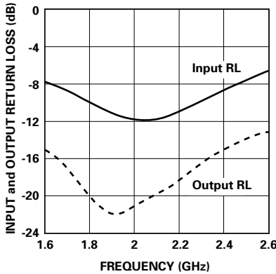
Figure 10. Input and Output Return Loss Results.
