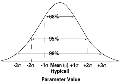
Figure 14. Normal Distribution.
