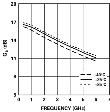
Figure 6. Associated Gain vs. Frequency and Temperature [1] .
