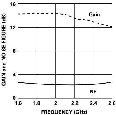
Figure 9. Gain and Noise Figure Results.
