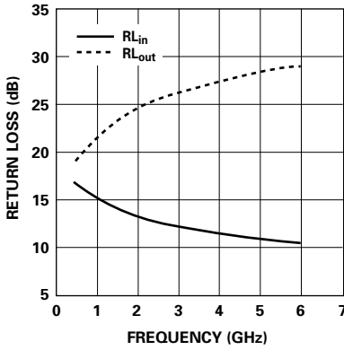
Figure 9. Return Losses at each Narrow Band Tuning.
