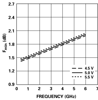
Figure 3. Minimum Noise Figure vs. Frequency and Voltage [1] .
